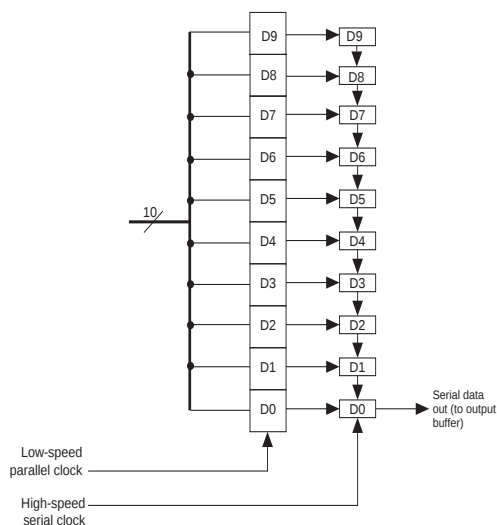
Figure 7. Serializer
