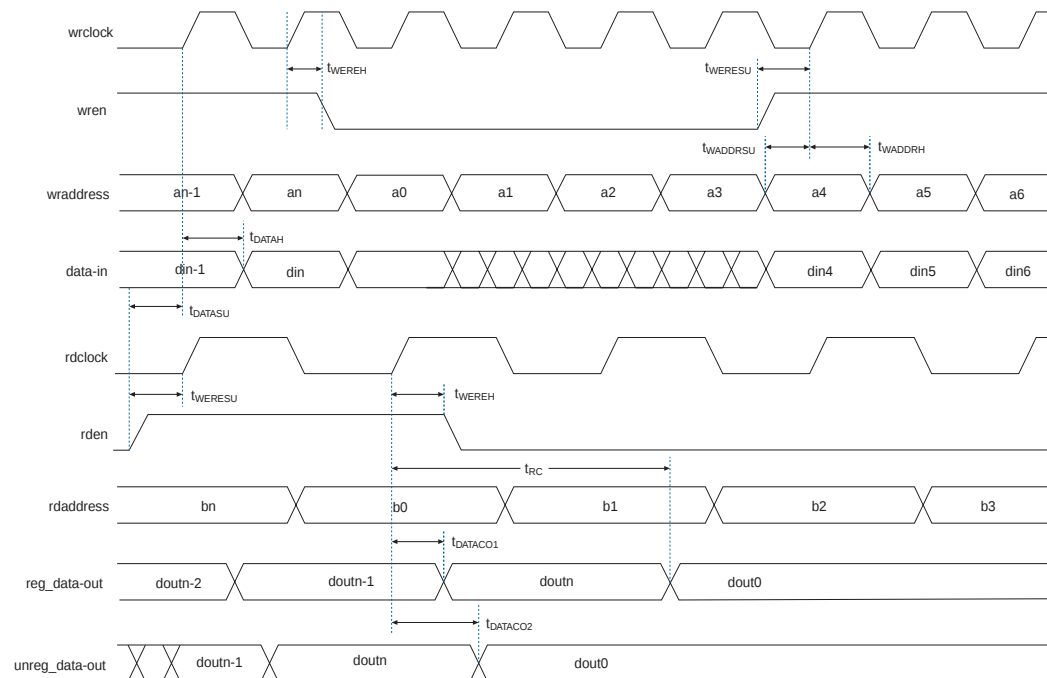
Figure 124. Dual-Port RAM Timing Microparameter Waveform
