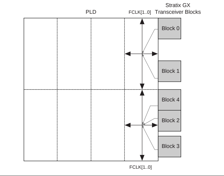
Figure 33. EP1SGX40 Receiver PLL Recovered Clock to Fast Regional Clock Connection
