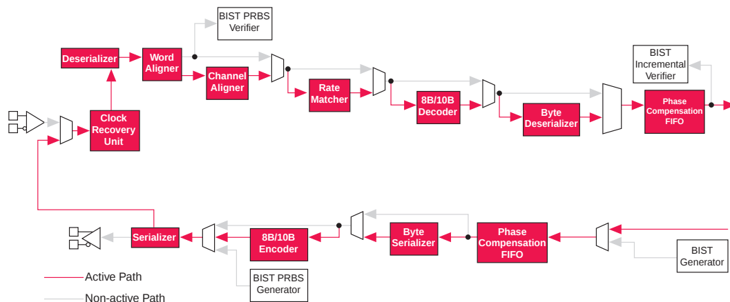
Figure 23. Data Path in Serial Loopback Mode
