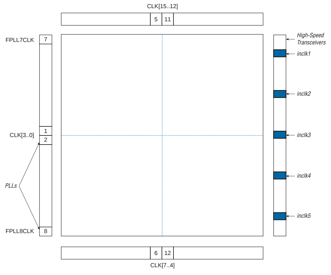
Figure 92. PLL Floorplan
