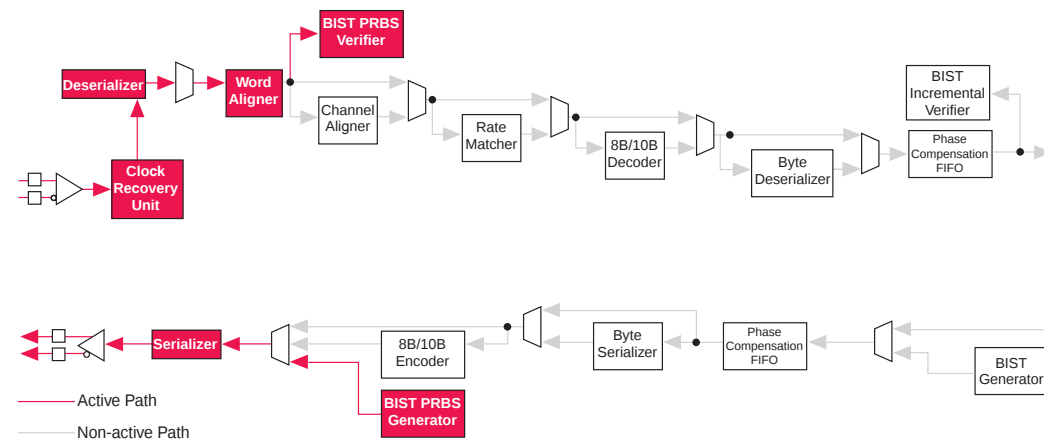
Figure 26. BIST PRBS Data Path
