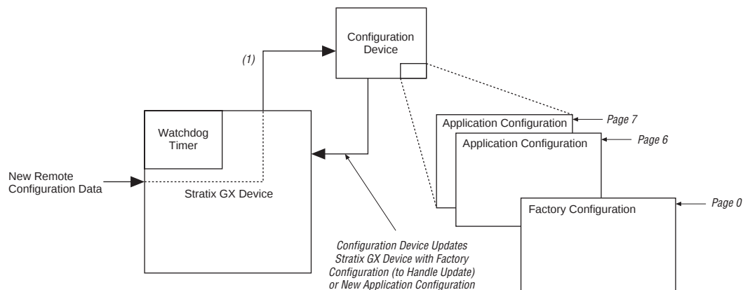
Figure 117. Stratix GX Device Remote Update
