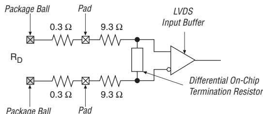
Figure 115. Differential Resistance of LVDS Differential Pin Pair ( R_D )
