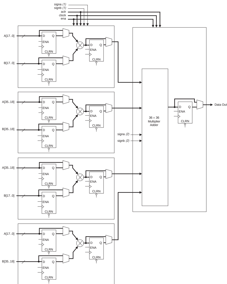
Figure 79. 36 \times 36 Multiply Mode
