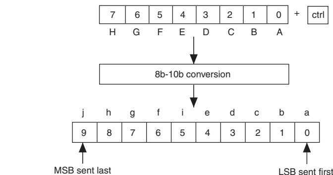
Figure 6. Encoding Process
