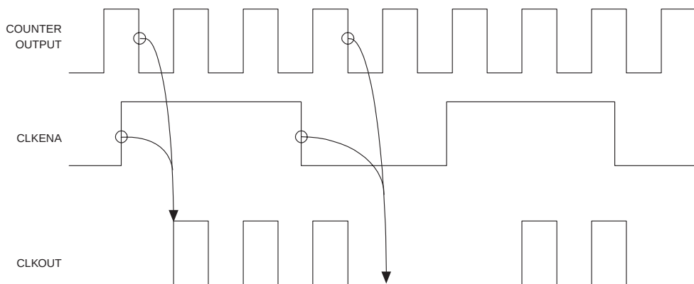
Figure 100. extclkena Signals
