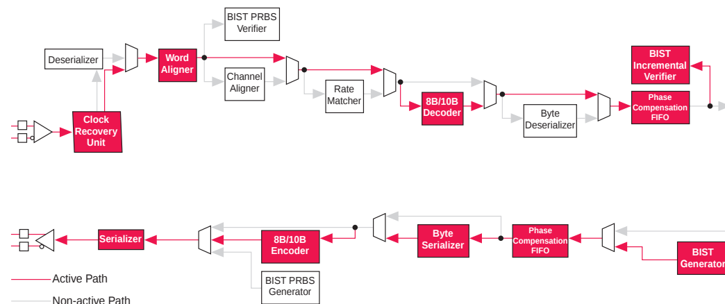
Figure 27. BIST Incremental Data Path
