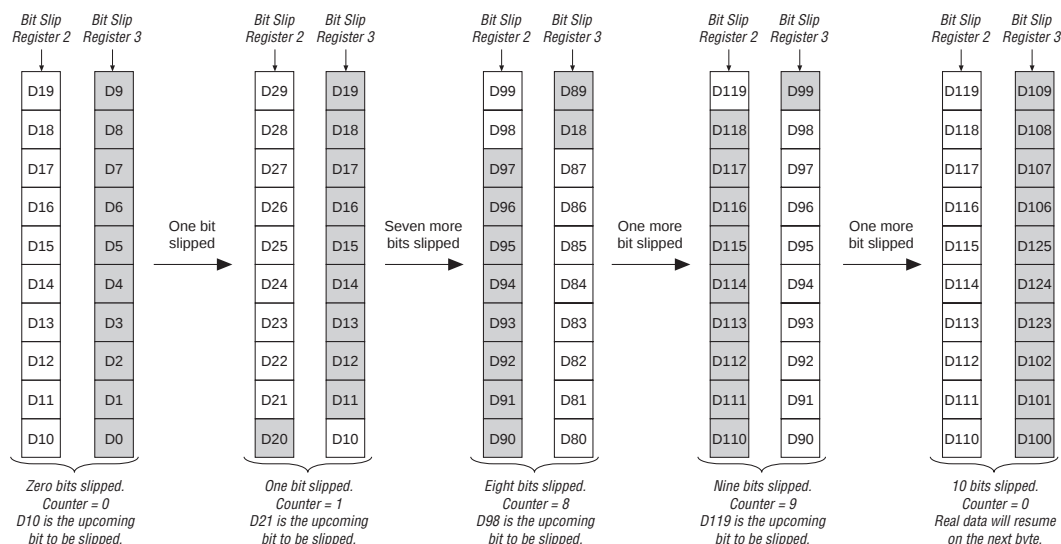
Figure 44. DPA Data Realigner
