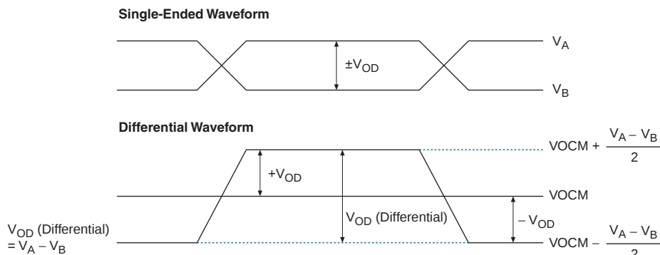
Figure 9. V_{OD} Differential
