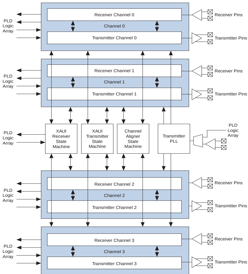
Figure 3. Stratix GX Transceiver Block
