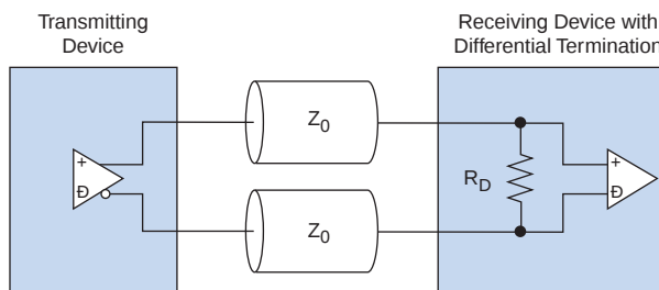
Figure 114. LVDS Input Differential On-Chip Termination
