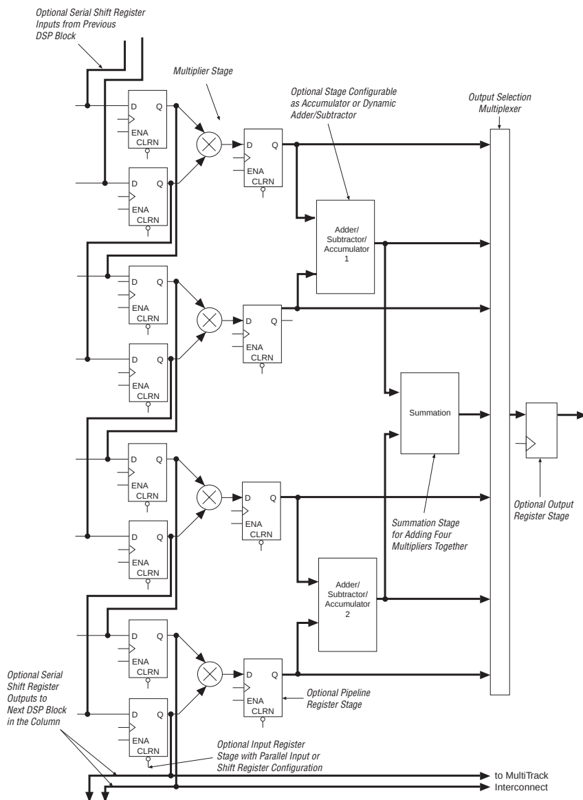
Figure 73. DSP Block Diagram for 18 \times 18 -Bit Configuration
