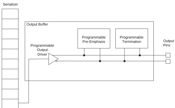
Figure 8. Output Buffer
